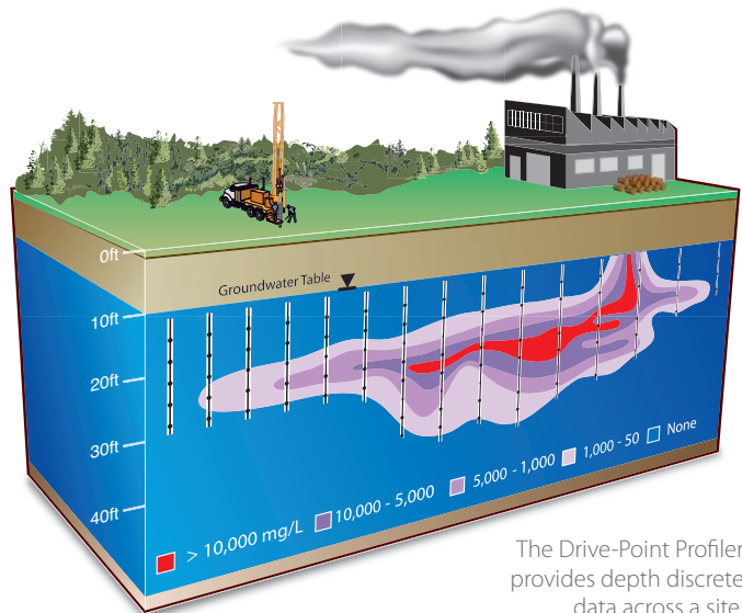
660 Drive-Point Profiler
